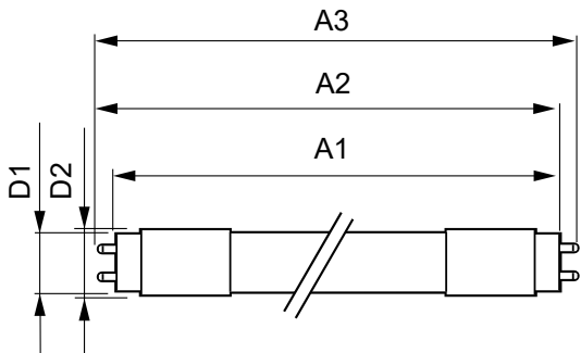
LEDtube 1200mm 16W 765
